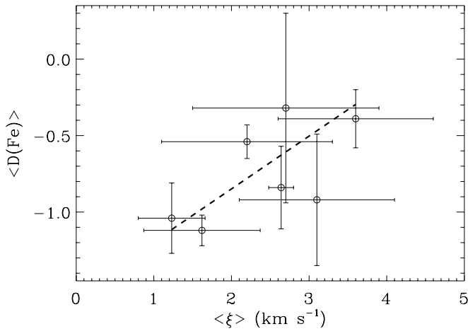
FIG. 21.—Distribution of the weighted mean values of turbulent velocity ( \xi ) and depletion of iron [ D(\text{Fe}) ] and magnesium [ D(\text{Mg}) ] for all clouds with more than one sight line having a turbulent velocity measurement. The errors are the dispersion about the weighted mean. The dashed line is a weighted minimum \chi^2 linear fit to the data. A clear correlation exists between cloud turbulent velocity and depletion for both elements, with a linear correlation coefficient r = 0.69 and a probability that the distribution could be drawn from an uncorrelated parent population of only P_c = 1.7\% for iron and r = 0.73 and P_c = 1.2\% for magnesium. It is likely that regions of high turbulence result from the dynamical interactions of clouds, which in turn produce shocks and heat any dust, returning metal ions from the dust to the gas phase.
