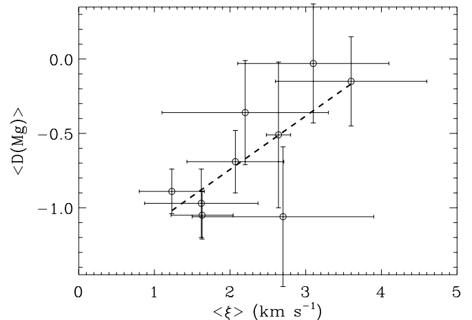
FIG. 21.—Distribution of the weighted mean values of turbulent velocity ( \xi ) and depletion of iron [ D(\text{Fe}) ] and magnesium [ D(\text{Mg}) ] for all clouds with more than one sight line having a turbulent velocity measurement. The errors are the dispersion about the weighted mean. The dashed line is a weighted minimum \chi^2 linear fit to the data. A clear correlation exists between cloud turbulent velocity and depletion for both elements, with a linear correlation coefficient r = 0.69 and a probability that the distribution could be drawn from an uncorrelated parent population of only P_c = 1.7\% for iron and r = 0.73 and P_c = 1.2\% for magnesium. It is likely that regions of high turbulence result from the dynamical interactions of clouds, which in turn produce shocks and heat any dust, returning metal ions from the dust to the gas phase.
