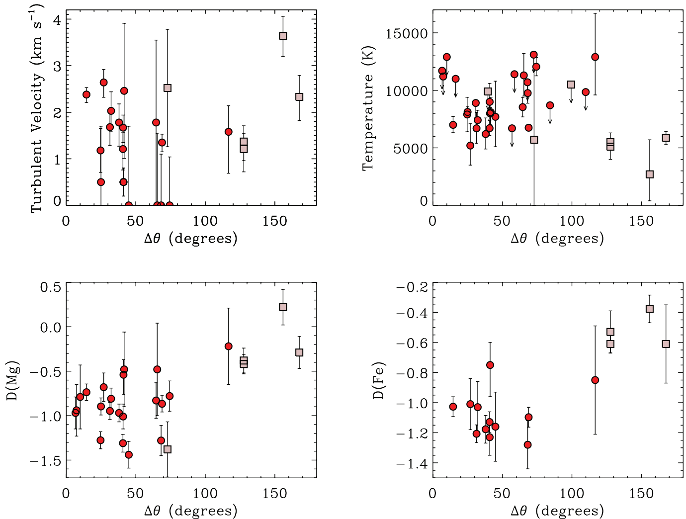
FIG. 23.— Comparison of LIC and G sight-line physical properties as a function of angular distance from the LIC downwind direction. Sight lines through each cloud are distinguished by color ( red : LIC; pale pink : G) and symbol ( circle : LIC; square : G). Since the G Cloud is in the upstream direction, all G Cloud sight lines are at high \Delta\theta . Except for one LIC value, all temperatures through the LIC are higher than the G Cloud temperatures. A correlation with angle is evident in the depletion of magnesium ( r = 0.63 , P_c = 0.012\% ) and iron ( r = 0.80 , P_c = 0.0041\% ).
