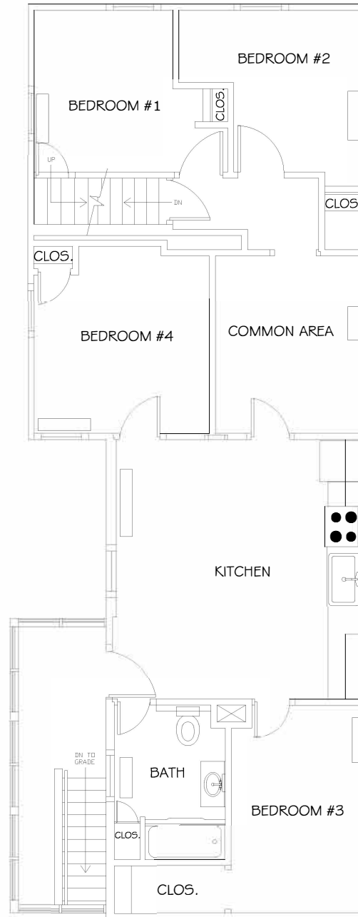
2ND FLOOR PLAN 12B FAIRVIEW AVENUE
