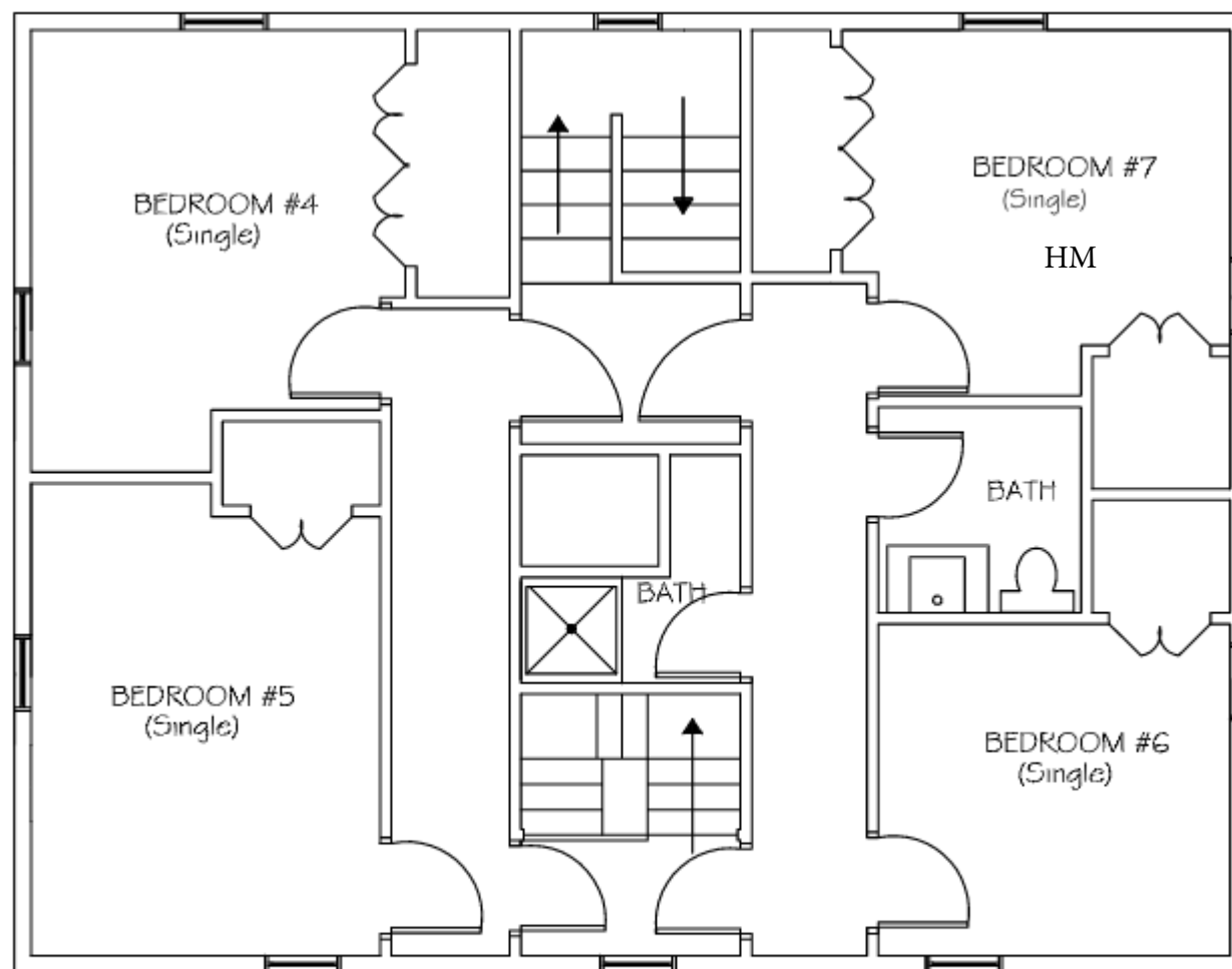
2ND FLOOR PLAN 227 PINE STREET
