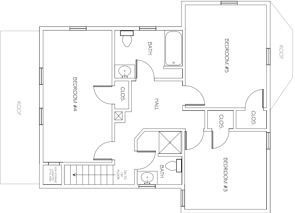
2ND FLOOR PLAN 142 CROSS STREET
