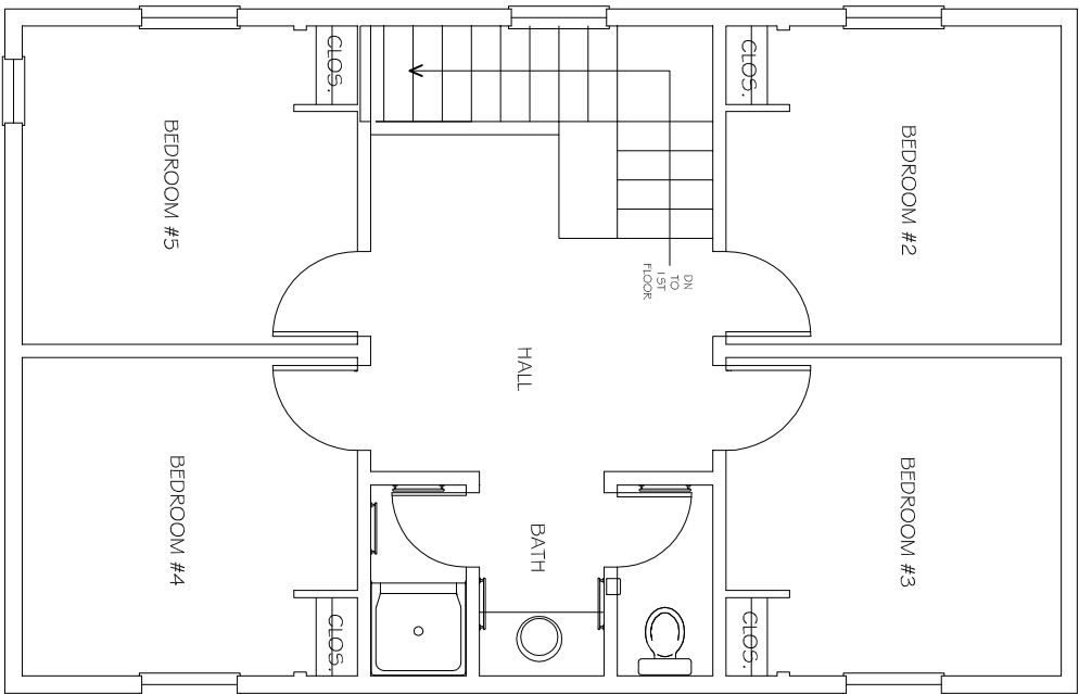
2ND FLOOR PLAN 20 C FOUNTAIN AVENUE
