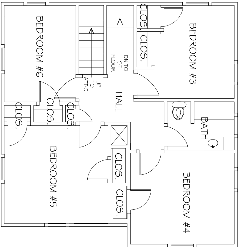
2ND FLOOR PLAN 88 HOME AVENUE
