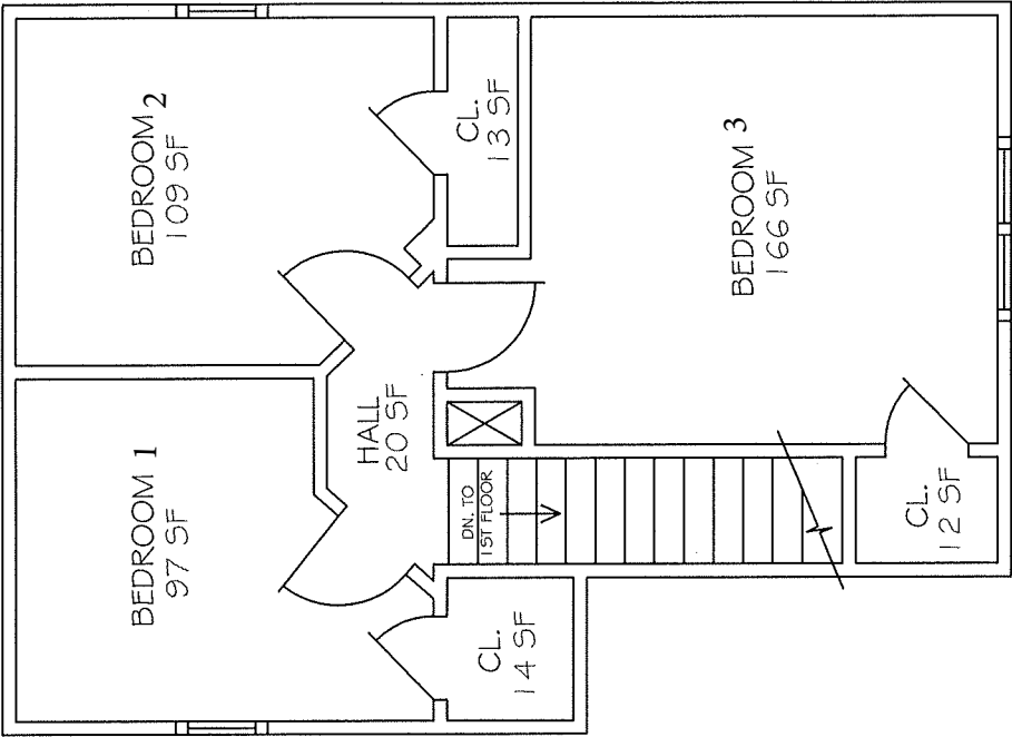
2ND FLOOR PLAN 9 HUBER AVENUE 529 GSF
