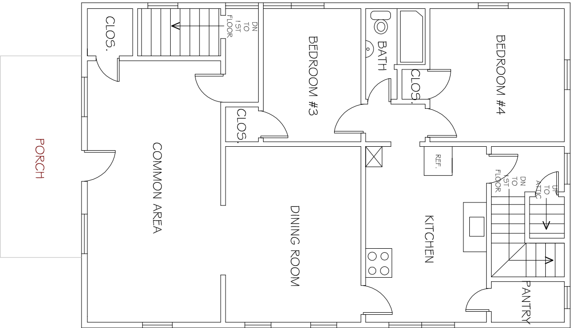
2ND FLOOR PLAN 122B KNOWLES AVENUE
