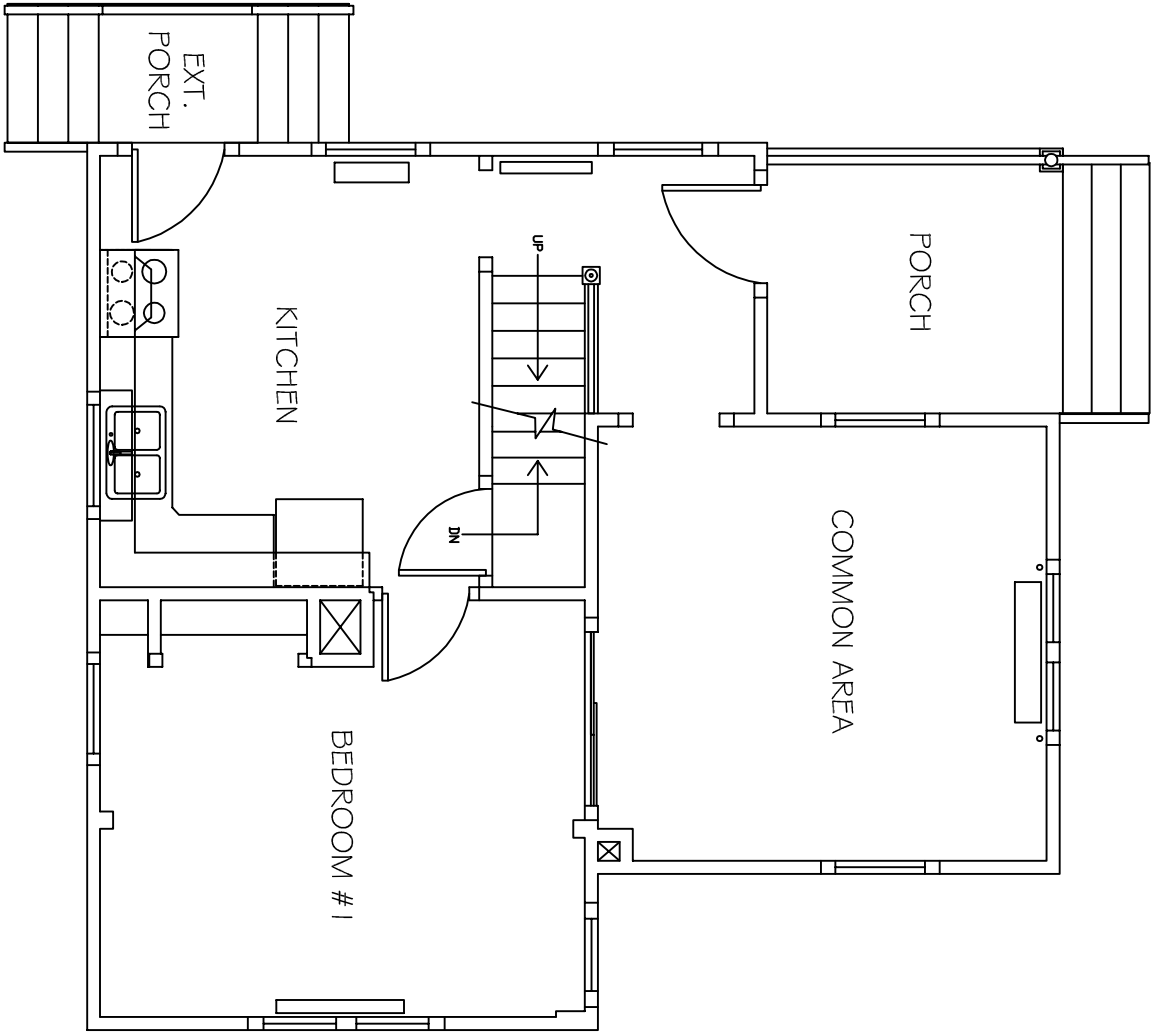
1ST FLOOR PLAN 273 PINE STREET
