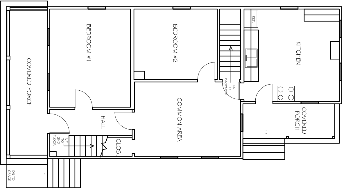
1ST FLOOR PLAN 8 WARREN STREET
