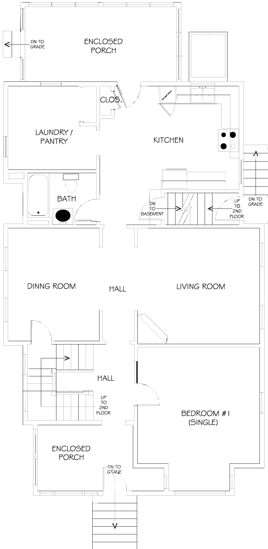
1ST FLOOR PLAN 59 PEARL STREET
